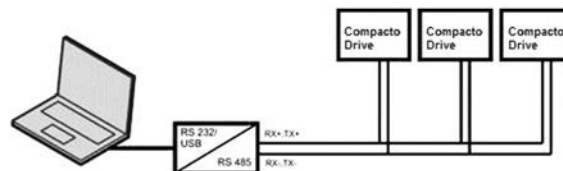
Parallel connections
